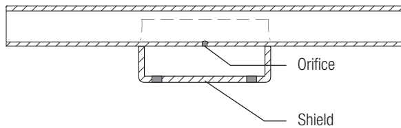
Cutaway view, cold weather configuration
